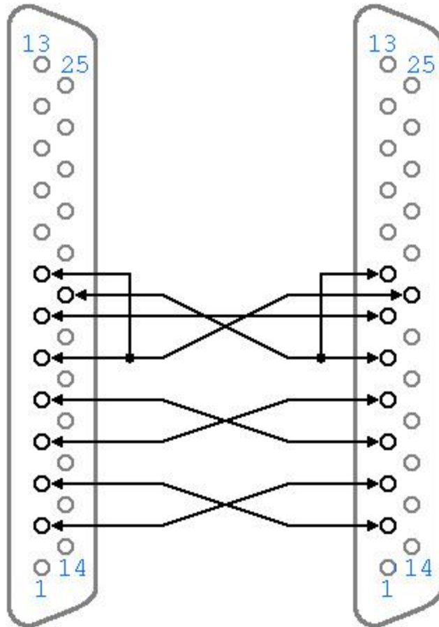
Null-modem wiring (DB-25 to DB-25)
